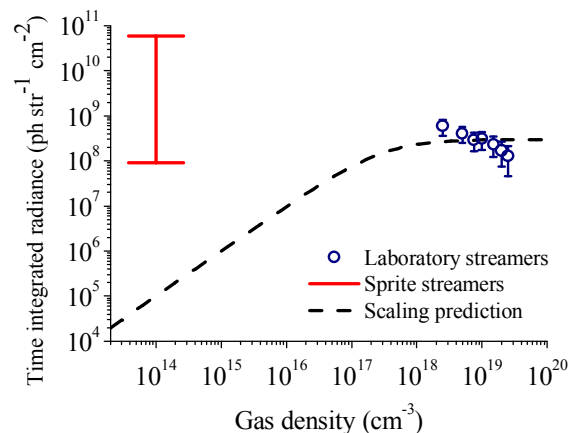
Figure 1 Time integrated radiance in air. Circles - experimental measurements in artificial air, point-plane geometry, dashed line - scaling law prediction. Red bar - sprite streamers, following observations by Stenbaek-Nielsen et al. [6].
